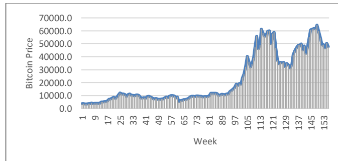
Figure 1. The plot of bitcoin price time series
